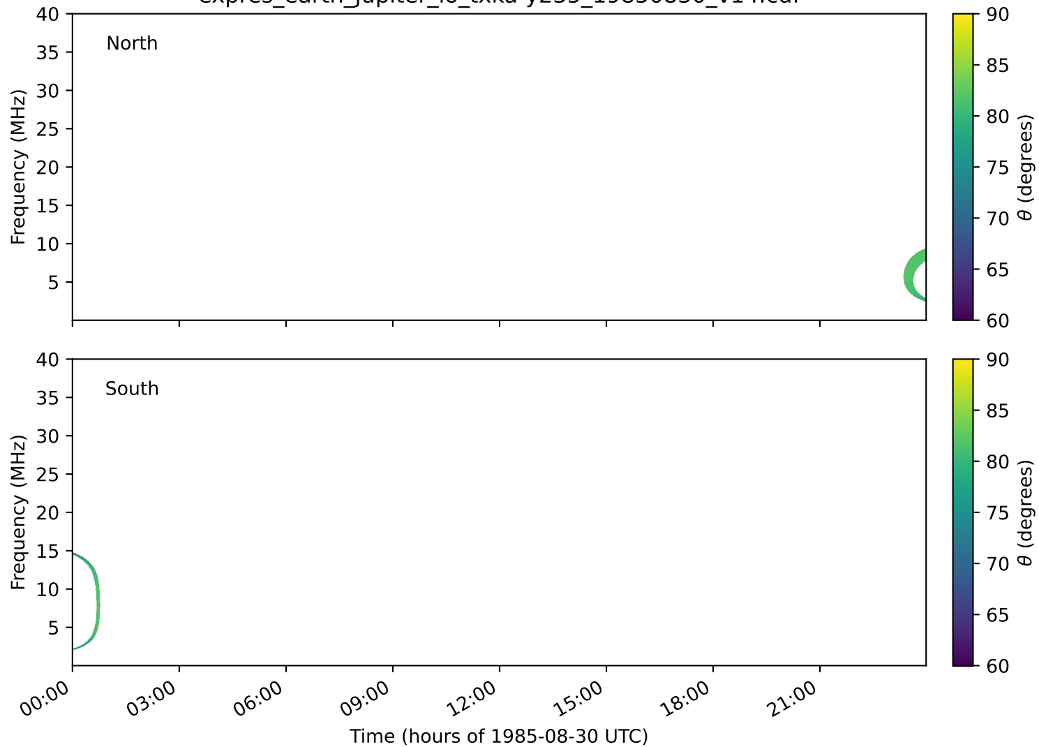
expres_earth_jupiter_io_txka-y235_19850830_v14.cdf
