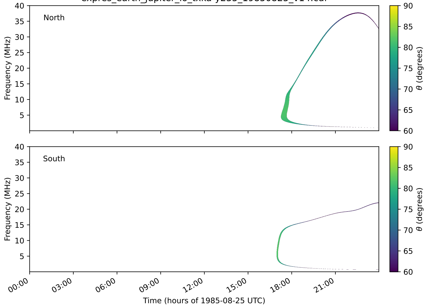
expres_earth_jupiter_io_txka-y235_19850825_v14.cdf
