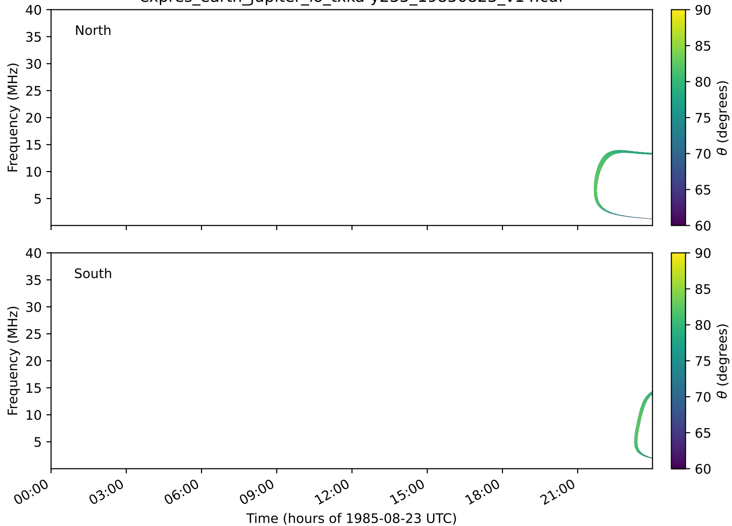
expres_earth_jupiter_io_txka-y235_19850823_v14.cdf
