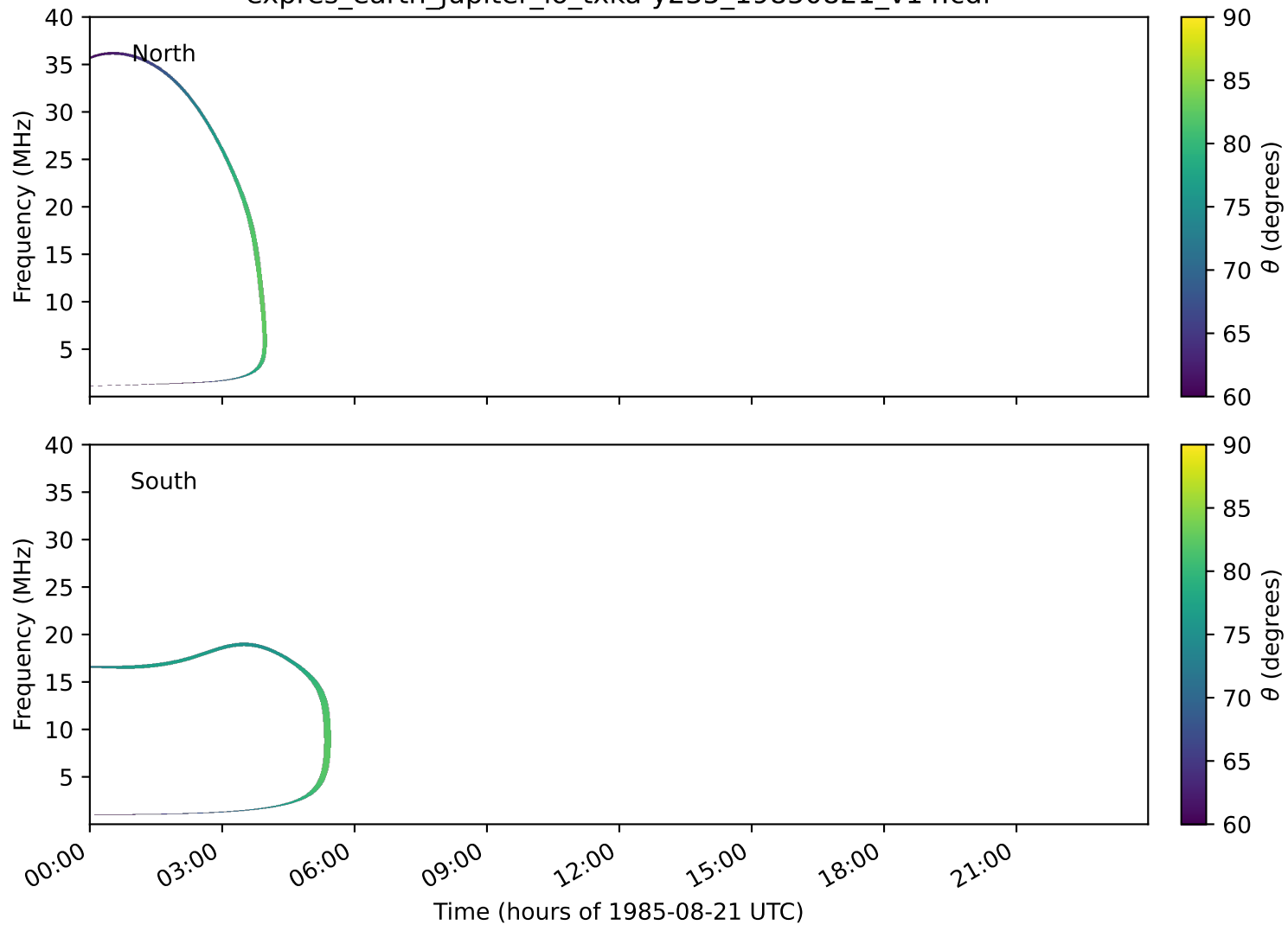
expres_earth_jupiter_io_txka-y235_19850821_v14.cdf
