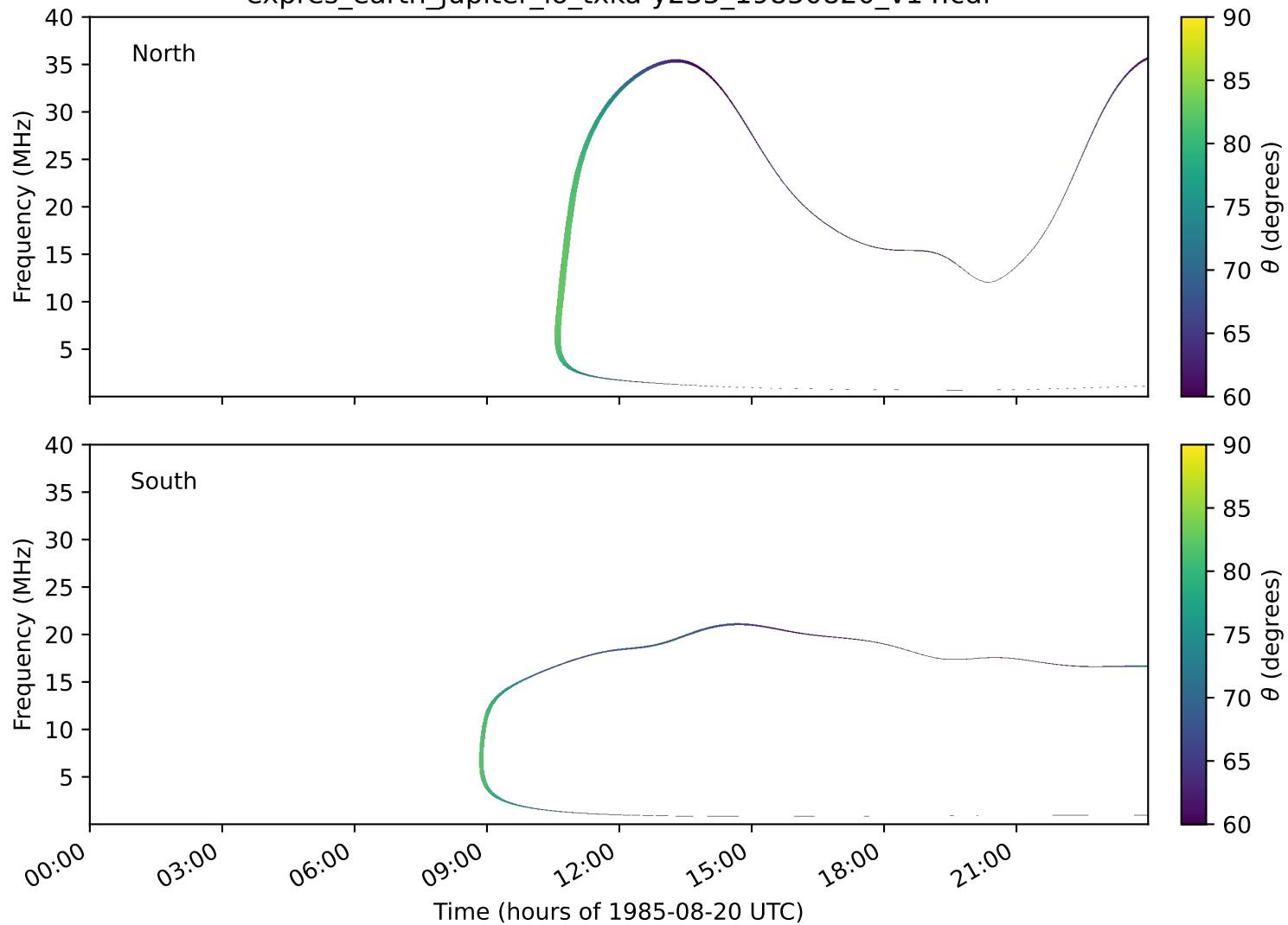
expres_earth_jupiter_io_txka-y235_19850820_v14.cdf
