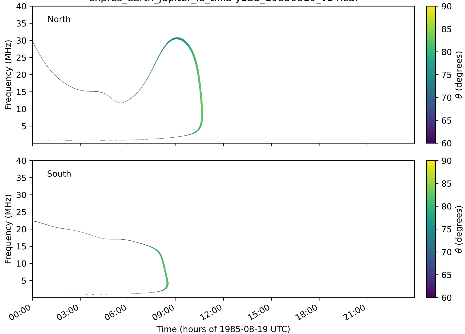
expres_earth_jupiter_io_txka-y235_19850819_v14.cdf
