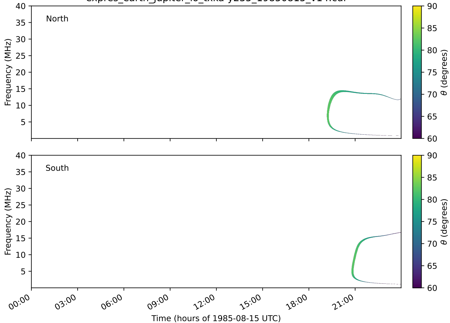
expres_earth_jupiter_io_txka-y235_19850815_v14.cdf
