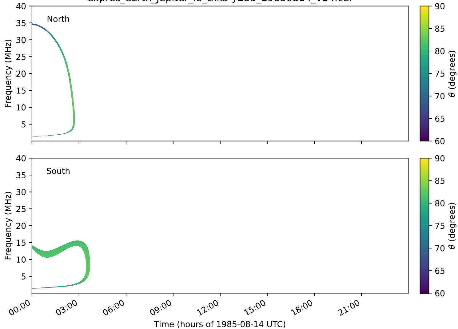
expres_earth_jupiter_io_txka-y235_19850814_v14.cdf
