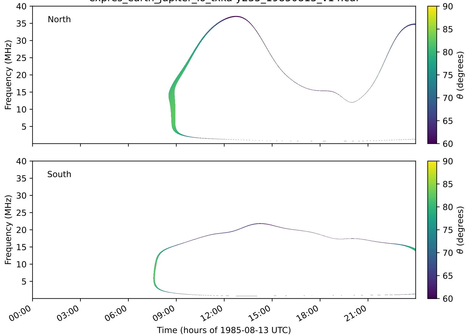
expres_earth_jupiter_io_txka-y235_19850813_v14.cdf
