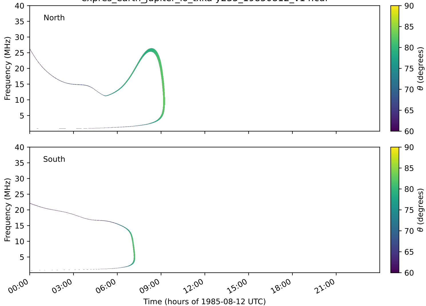
expres_earth_jupiter_io_txka-y235_19850812_v14.cdf
