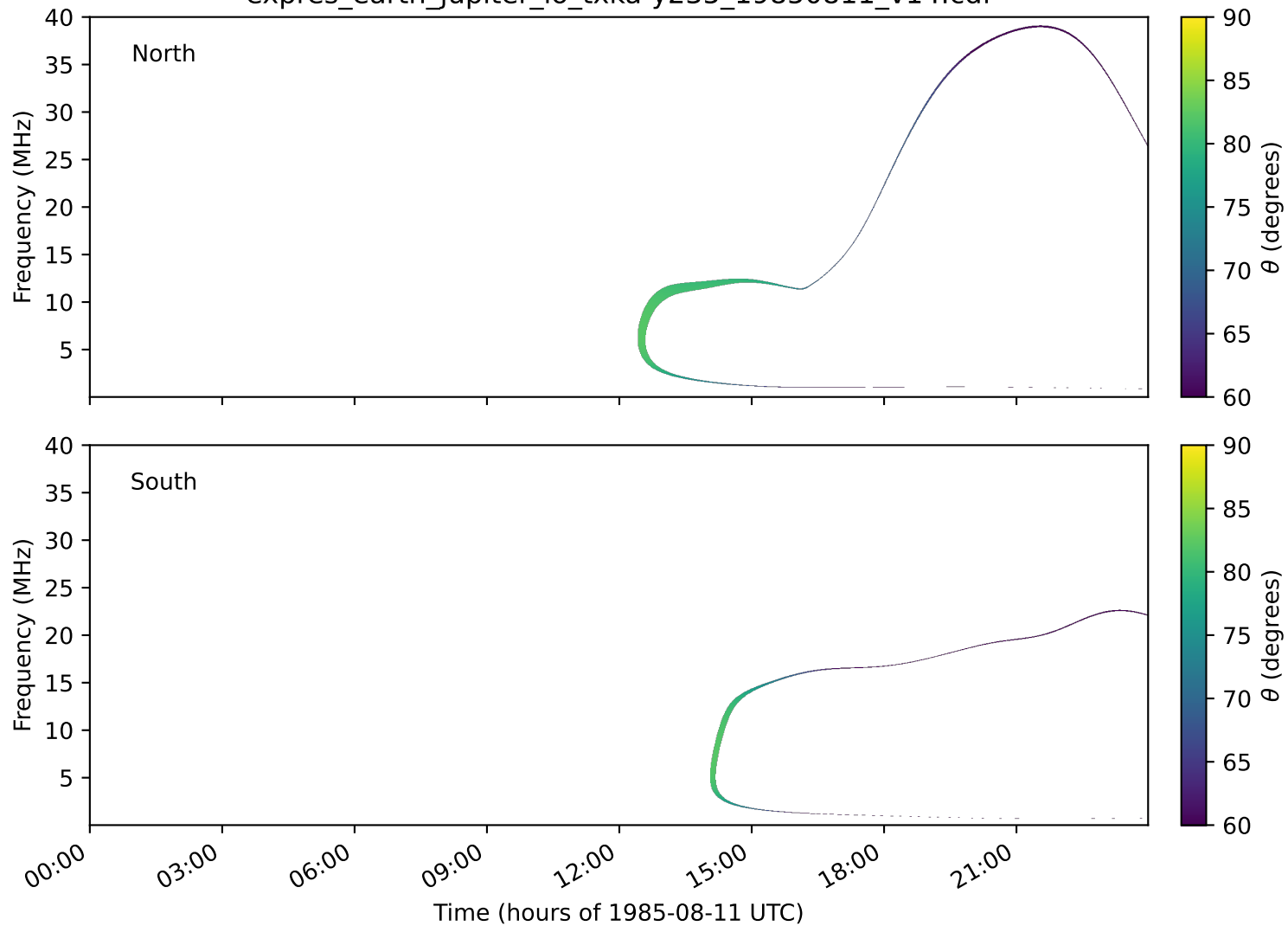
expres_earth_jupiter_io_txka-y235_19850811_v14.cdf
