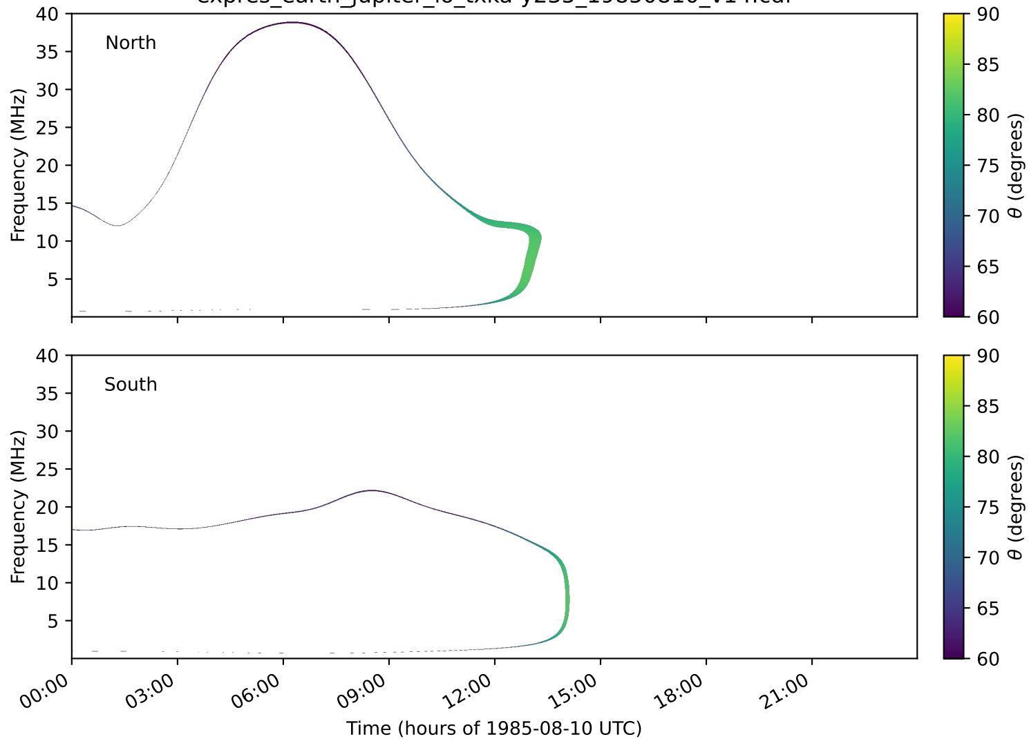
expres_earth_jupiter_io_txka-y235_19850810_v14.cdf
