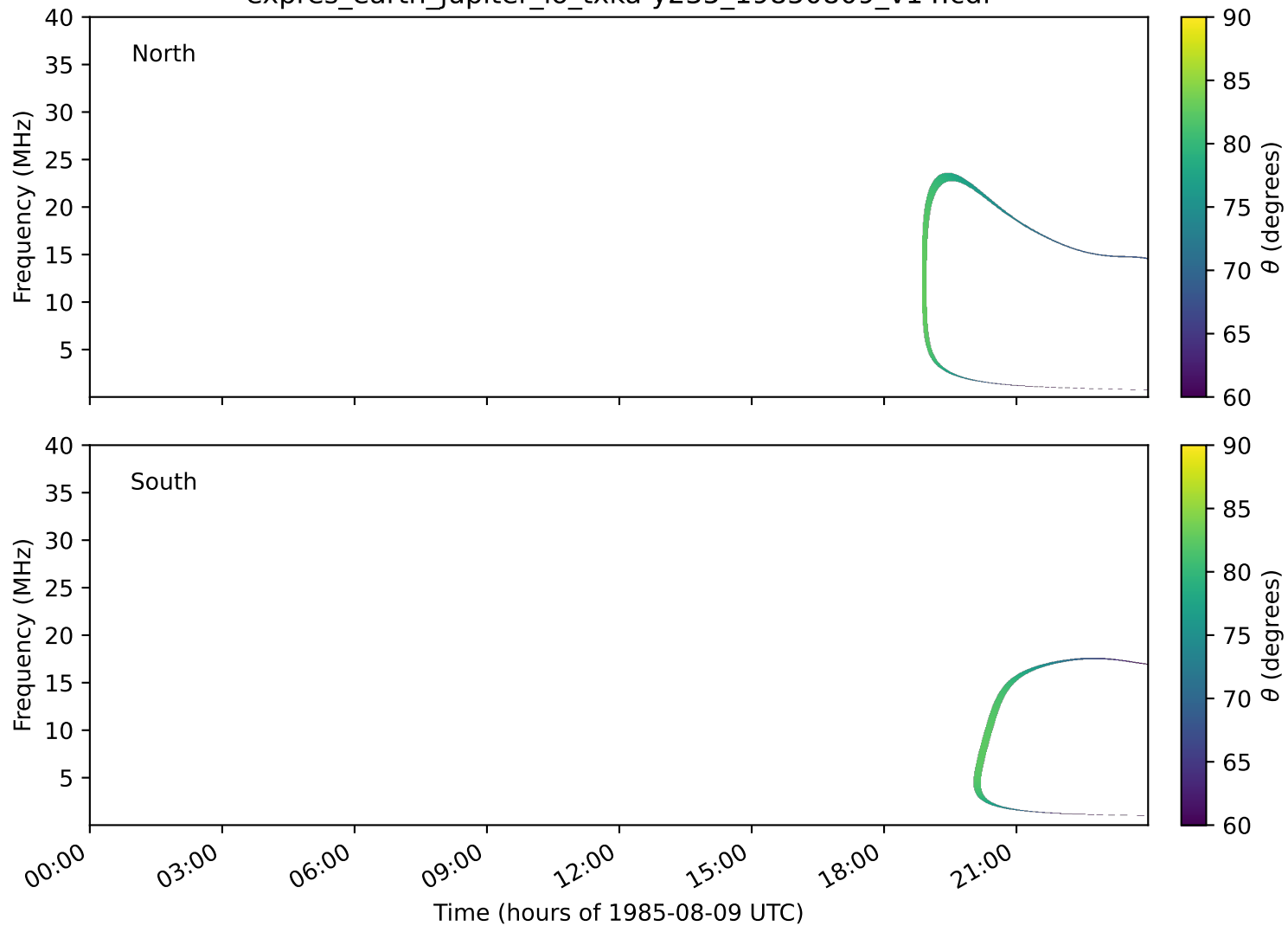
expres_earth_jupiter_io_txka-y235_19850809_v14.cdf
