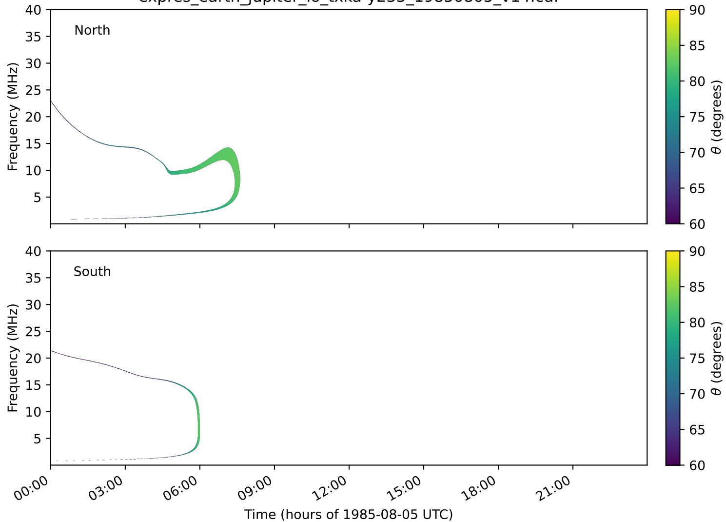
expres_earth_jupiter_io_txka-y235_19850805_v14.cdf
