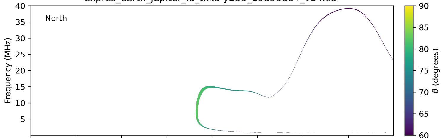
expres_earth_jupiter_io_txka-y235_19850804_v14.cdf
