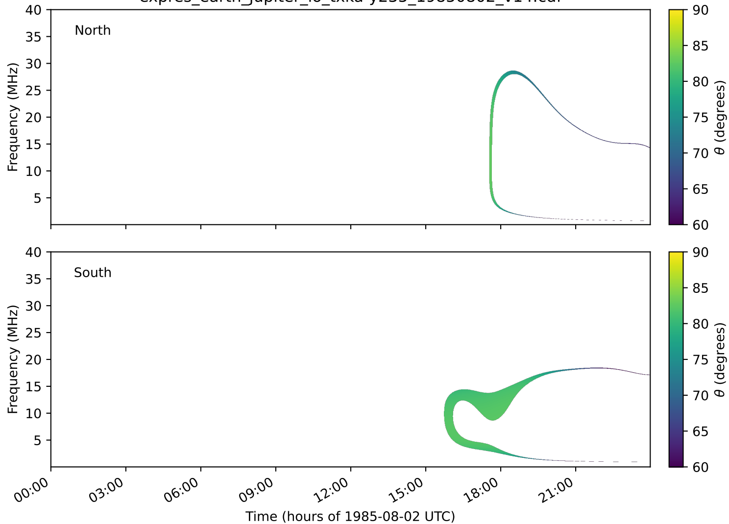
expres_earth_jupiter_io_txka-y235_19850802_v14.cdf
