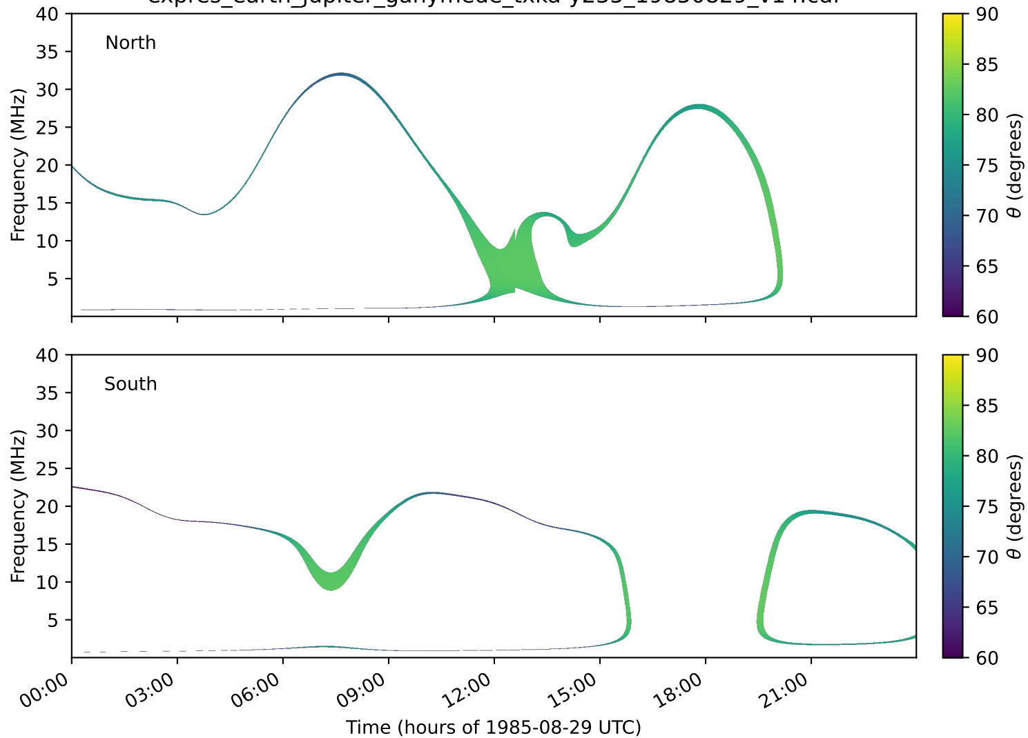
expres_earth_jupiter_ganymede_txka-y235_19850829_v14.cdf
