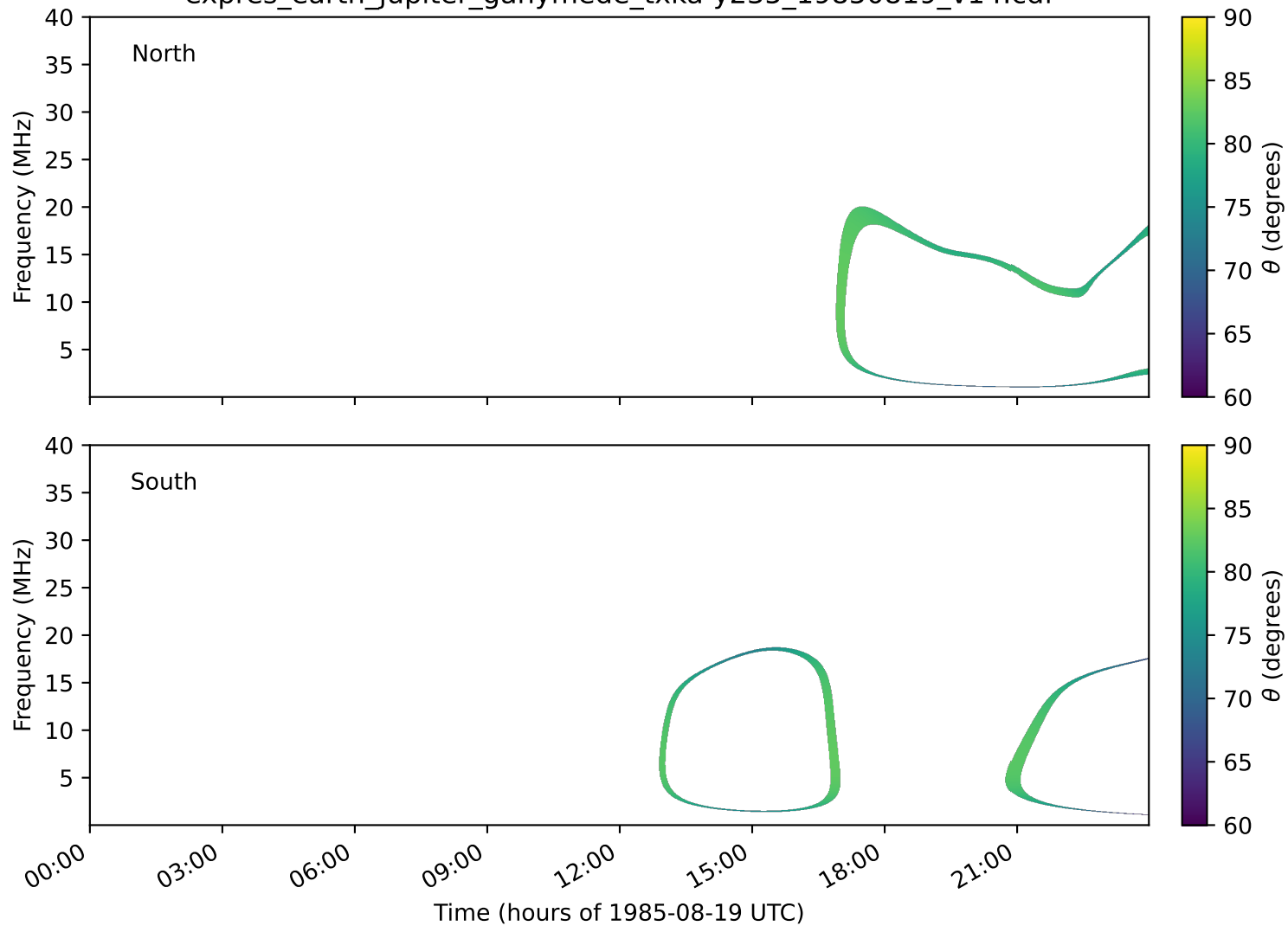
expres_earth_jupiter_ganymede_txka-y235_19850819_v14.cdf
