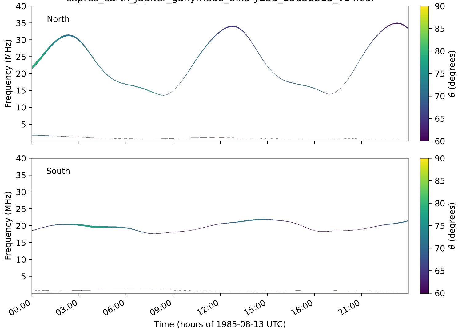
expres_earth_jupiter_ganymede_txka-y235_19850813_v14.cdf
