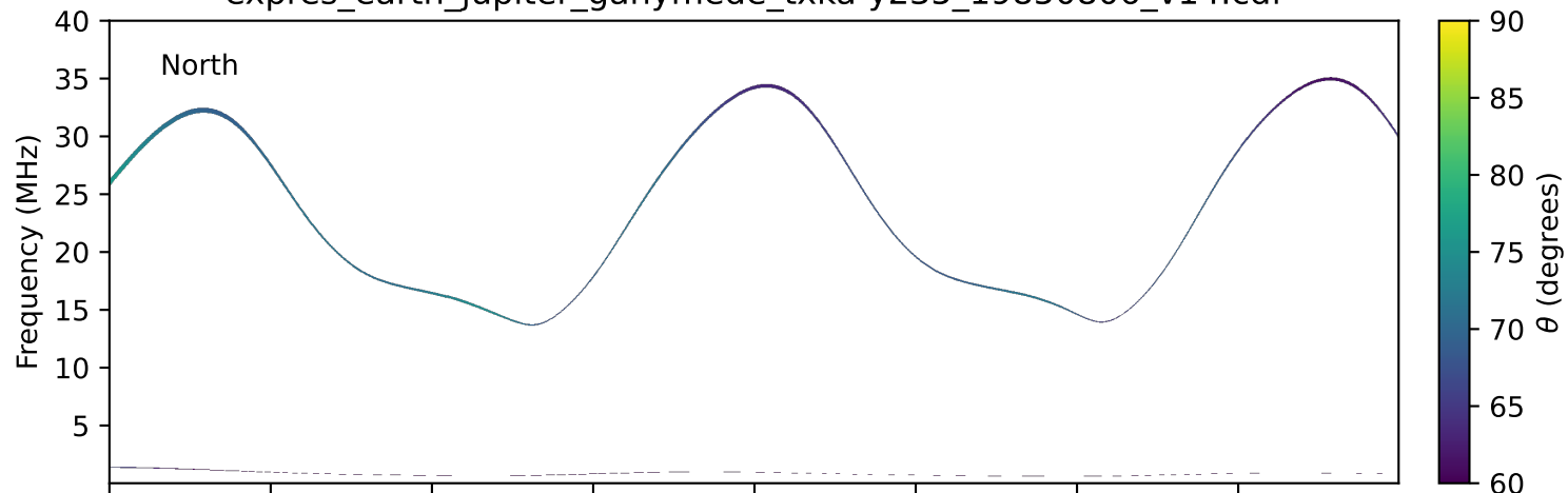
expres_earth_jupiter_ganymede_txka-y235_19850806_v14.cdf
