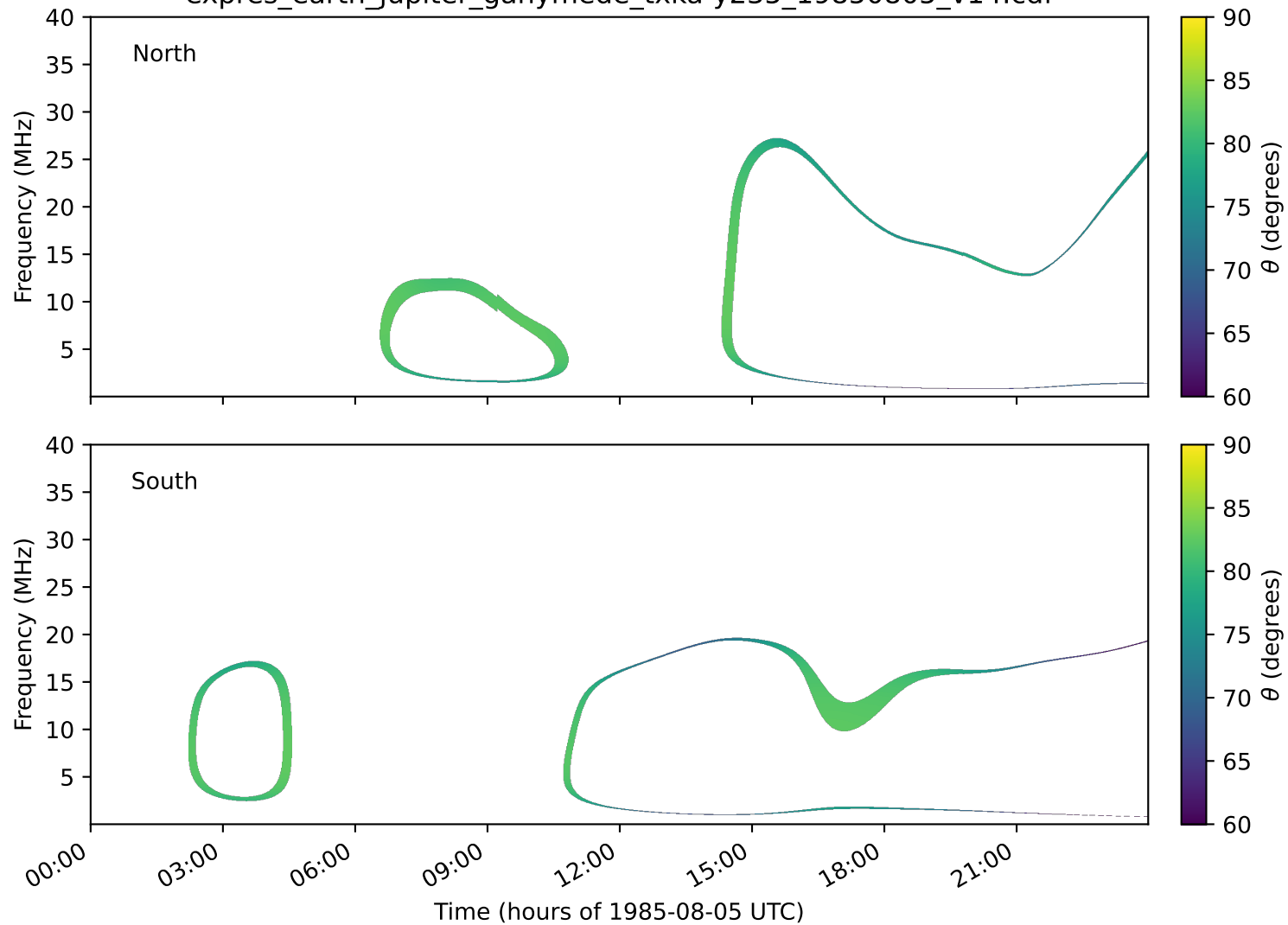
expres_earth_jupiter_ganymede_txka-y235_19850805_v14.cdf
