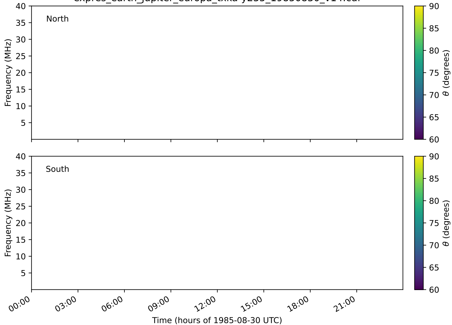
expres_earth_jupiter_europa_txka-y235_19850830_v14.cdf
