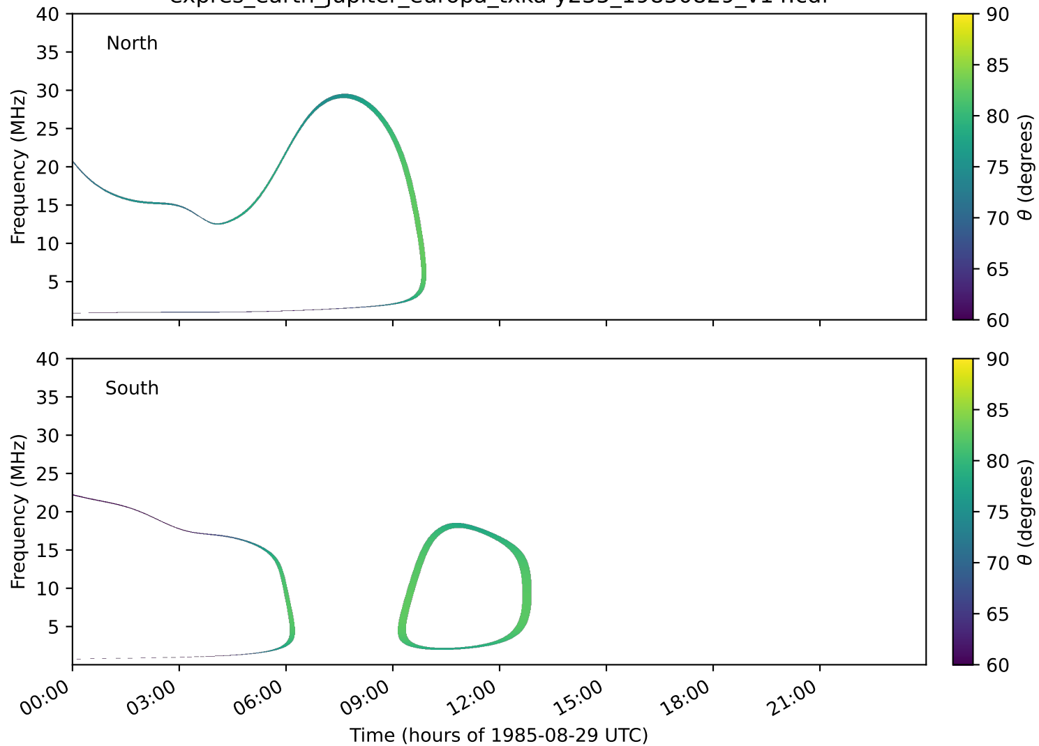
expres_earth_jupiter_europa_txka-y235_19850829_v14.cdf
