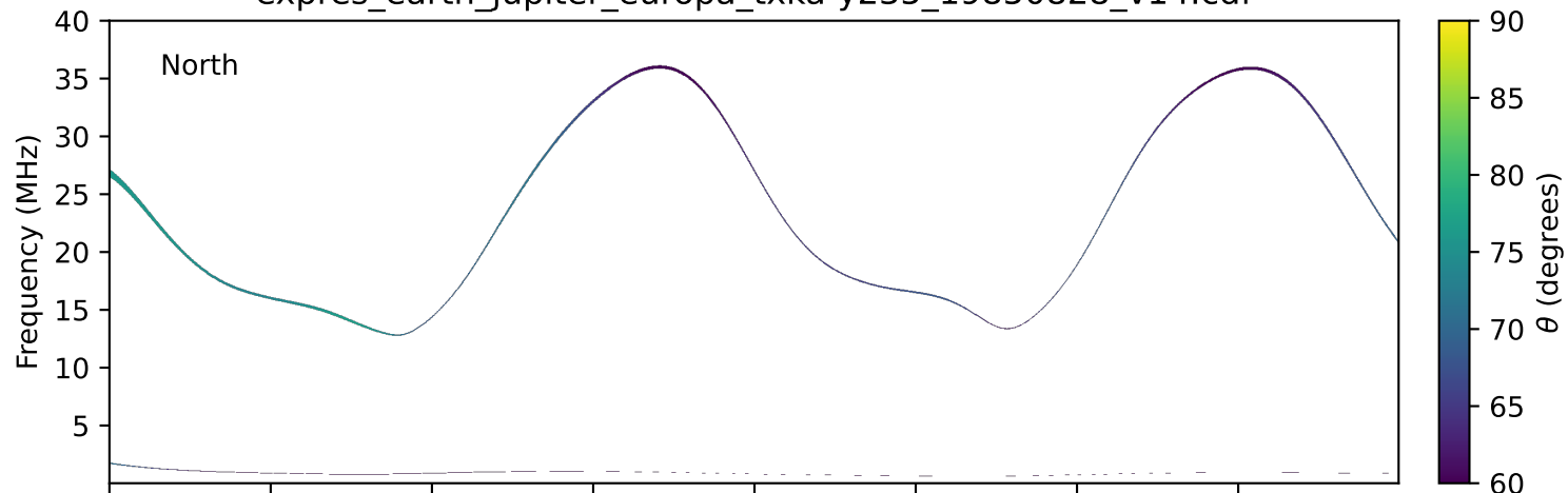
expres_earth_jupiter_europa_txka-y235_19850828_v14.cdf
