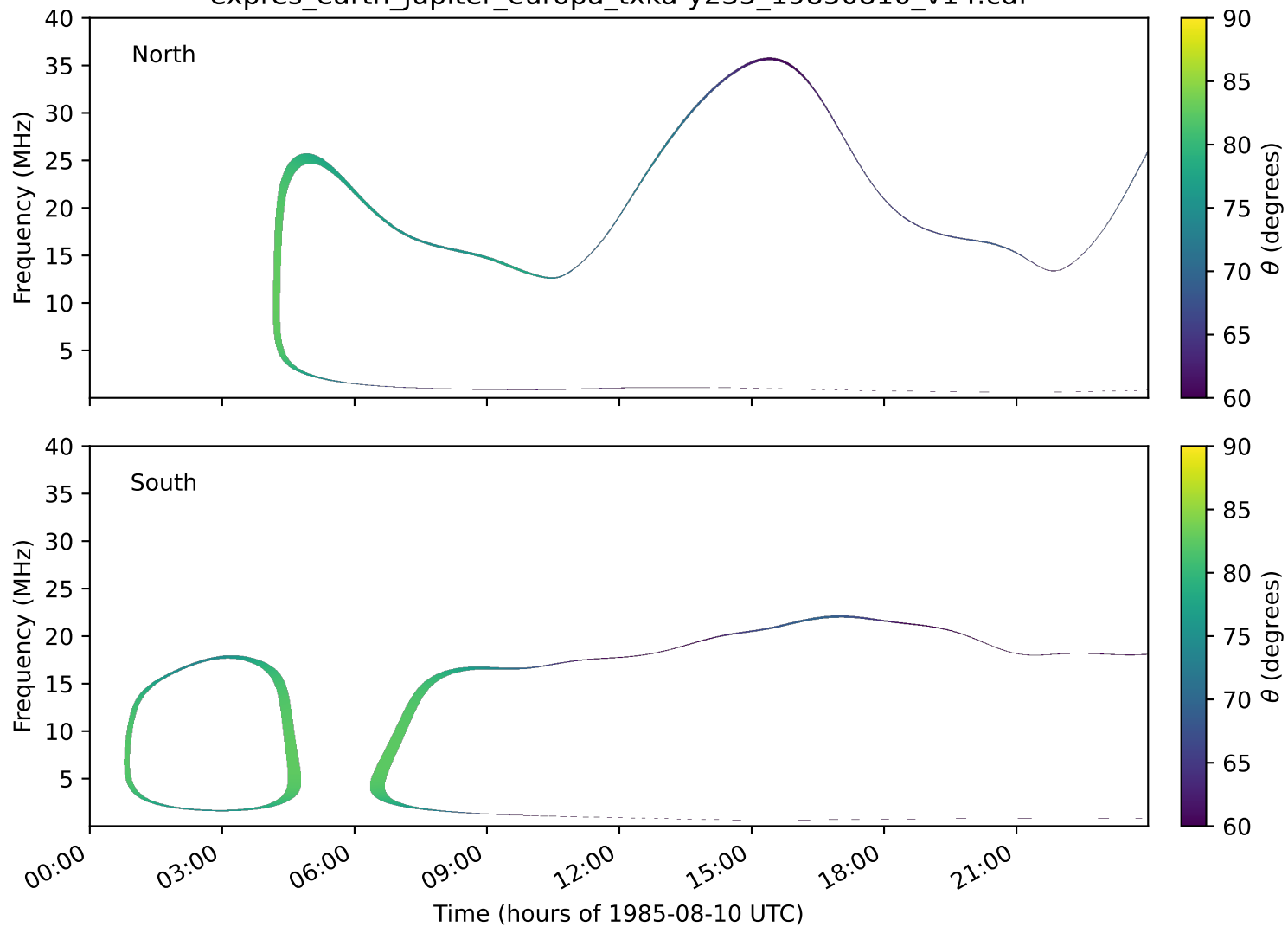
expres_earth_jupiter_europa_txka-y235_19850810_v14.cdf
