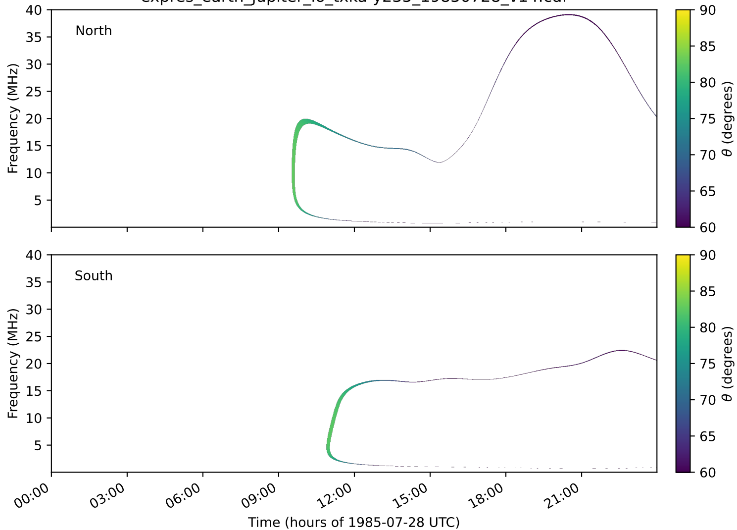
expres_earth_jupiter_io_txka-y235_19850728_v14.cdf
