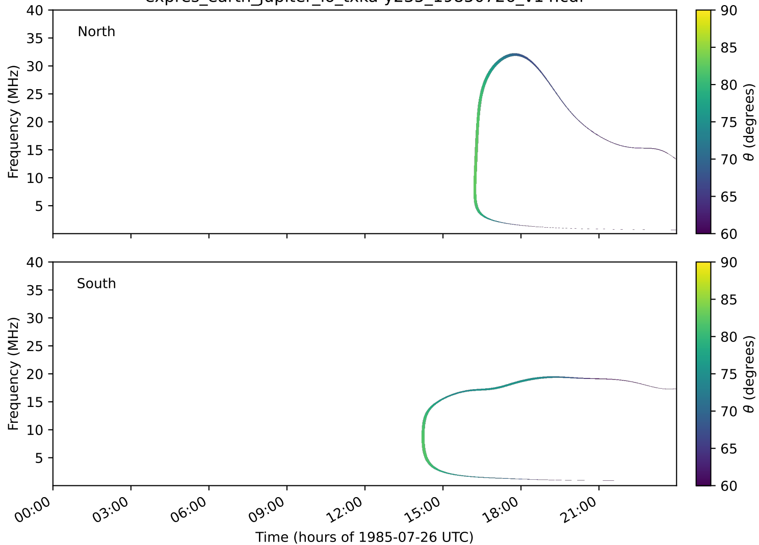
expres_earth_jupiter_io_txka-y235_19850726_v14.cdf
