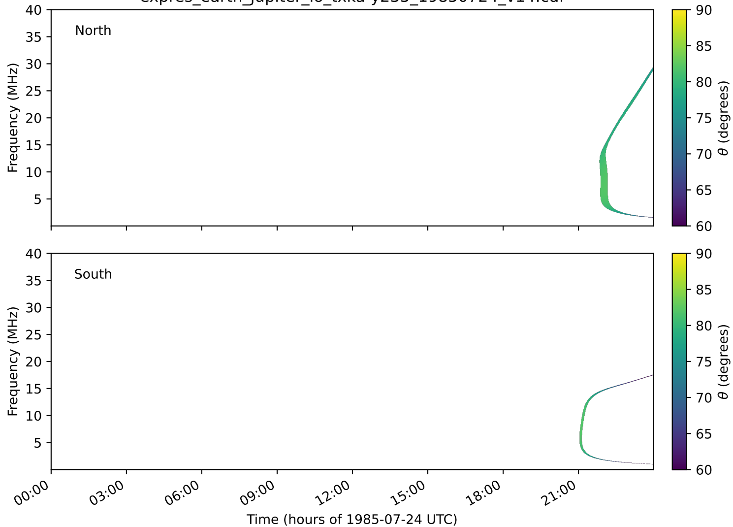
expres_earth_jupiter_io_txka-y235_19850724_v14.cdf
