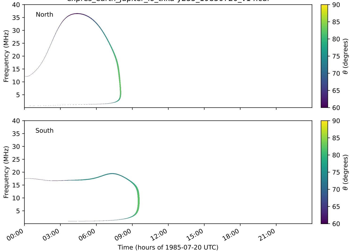
expres_earth_jupiter_io_txka-y235_19850720_v14.cdf
