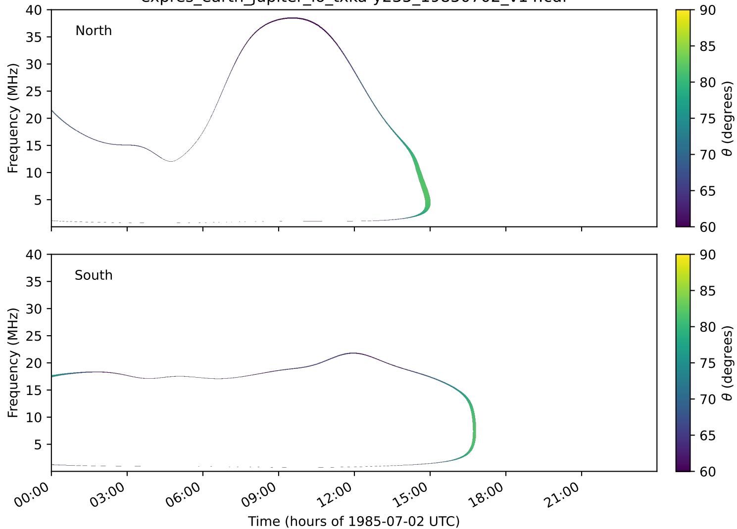
expres_earth_jupiter_io_txka-y235_19850702_v14.cdf
