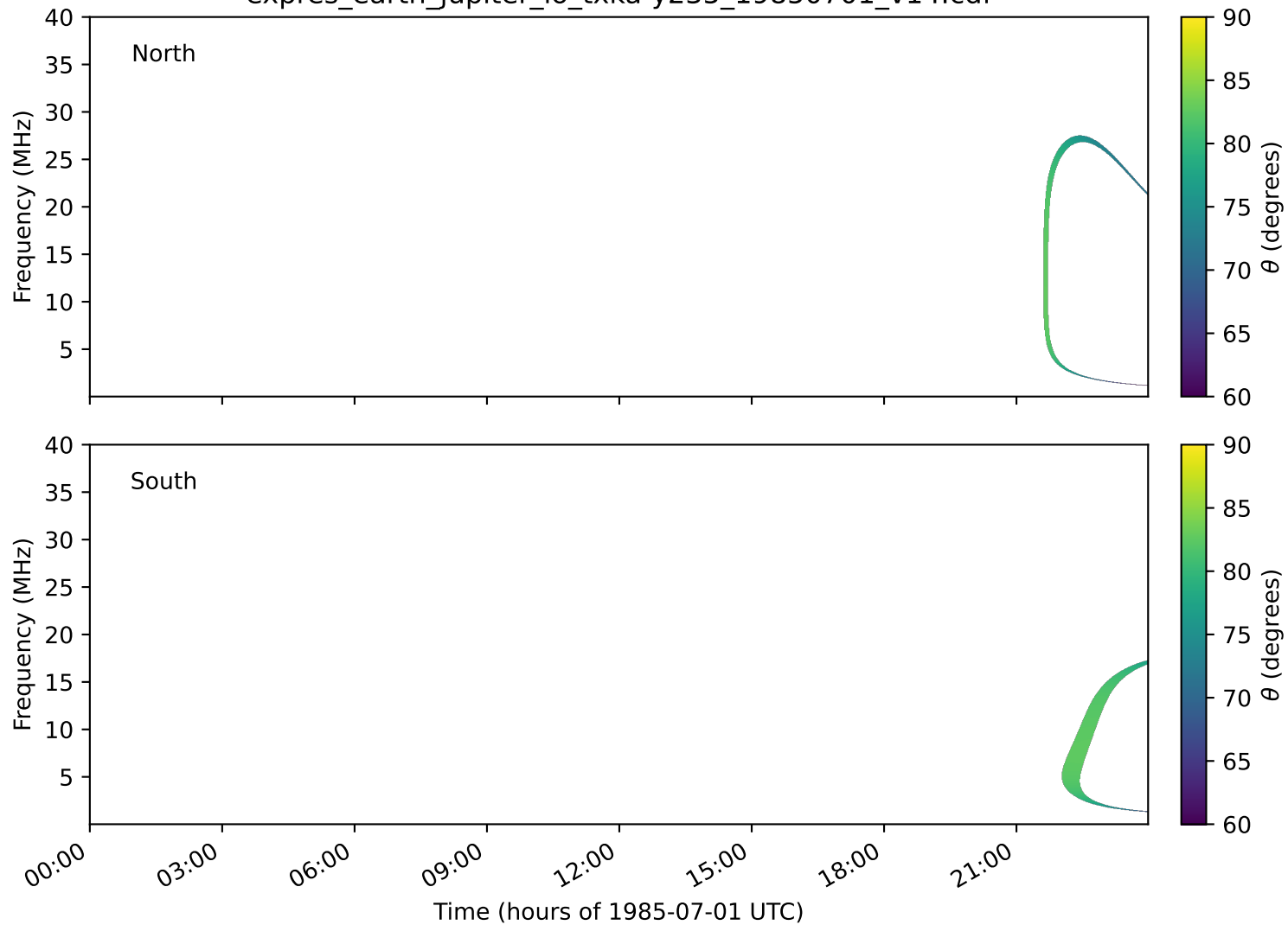
expres_earth_jupiter_io_txka-y235_19850701_v14.cdf
