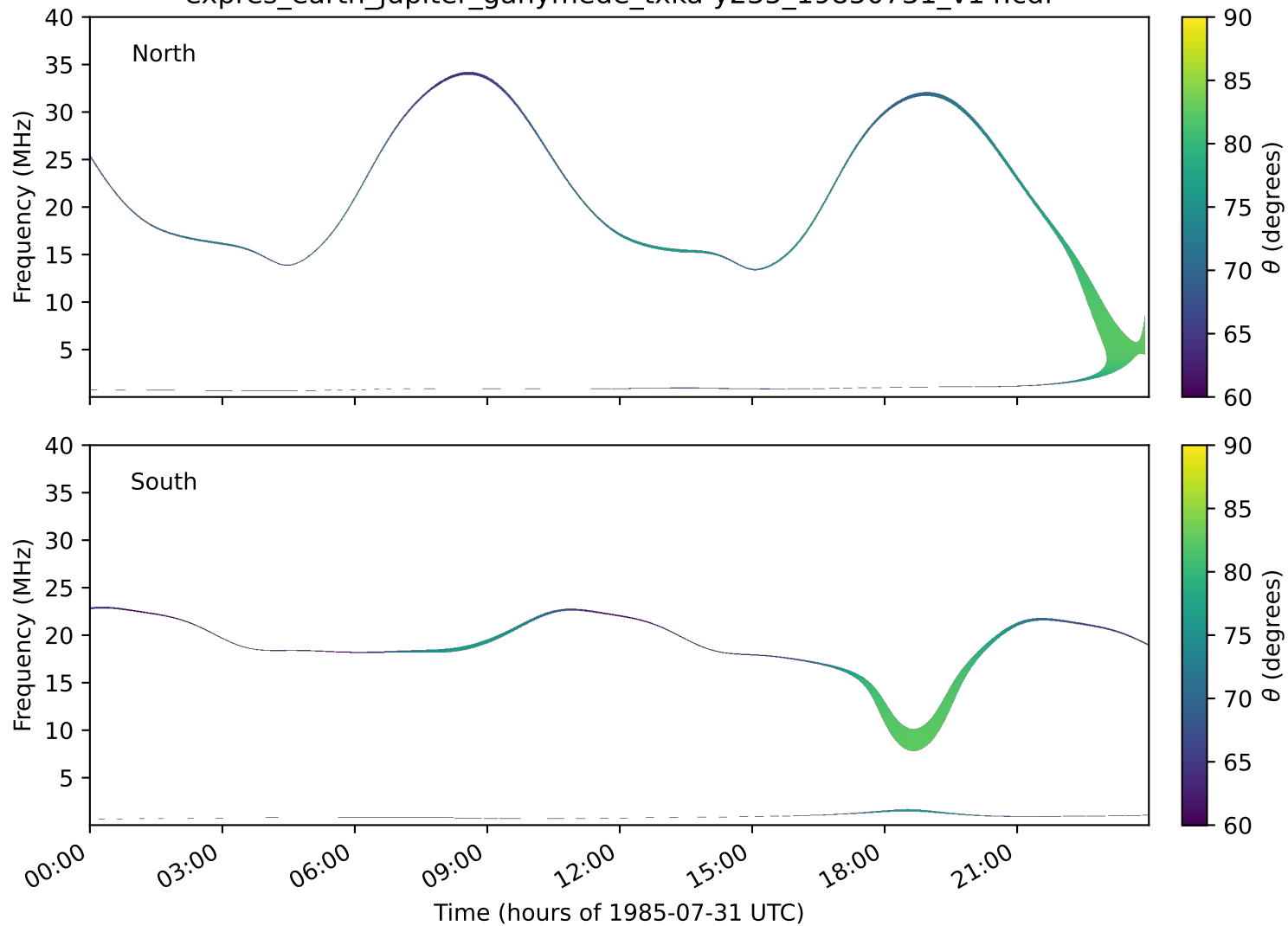
expres_earth_jupiter_ganymede_txka-y235_19850731_v14.cdf
