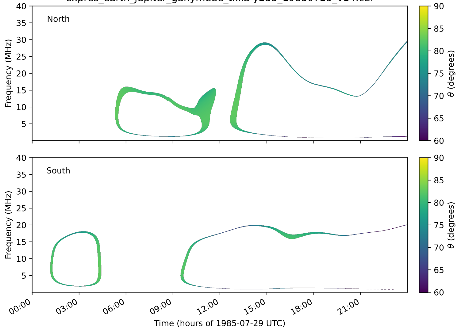
expres_earth_jupiter_ganymede_txka-y235_19850729_v14.cdf
