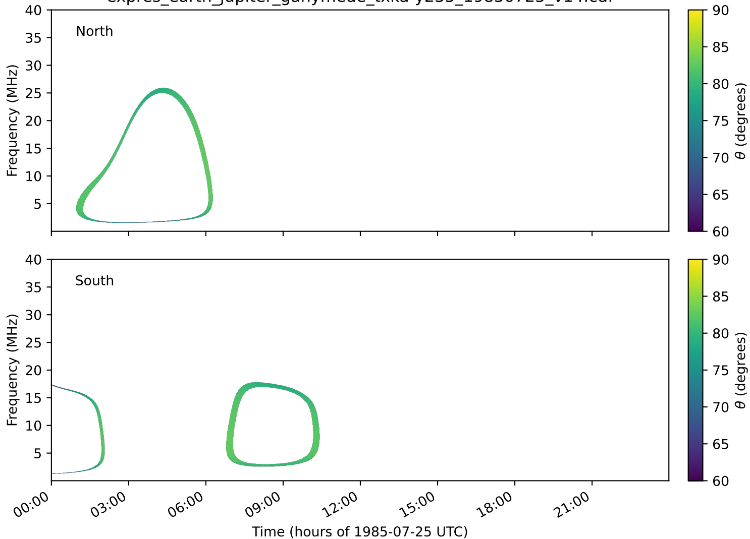
expres_earth_jupiter_ganymede_txka-y235_19850725_v14.cdf
