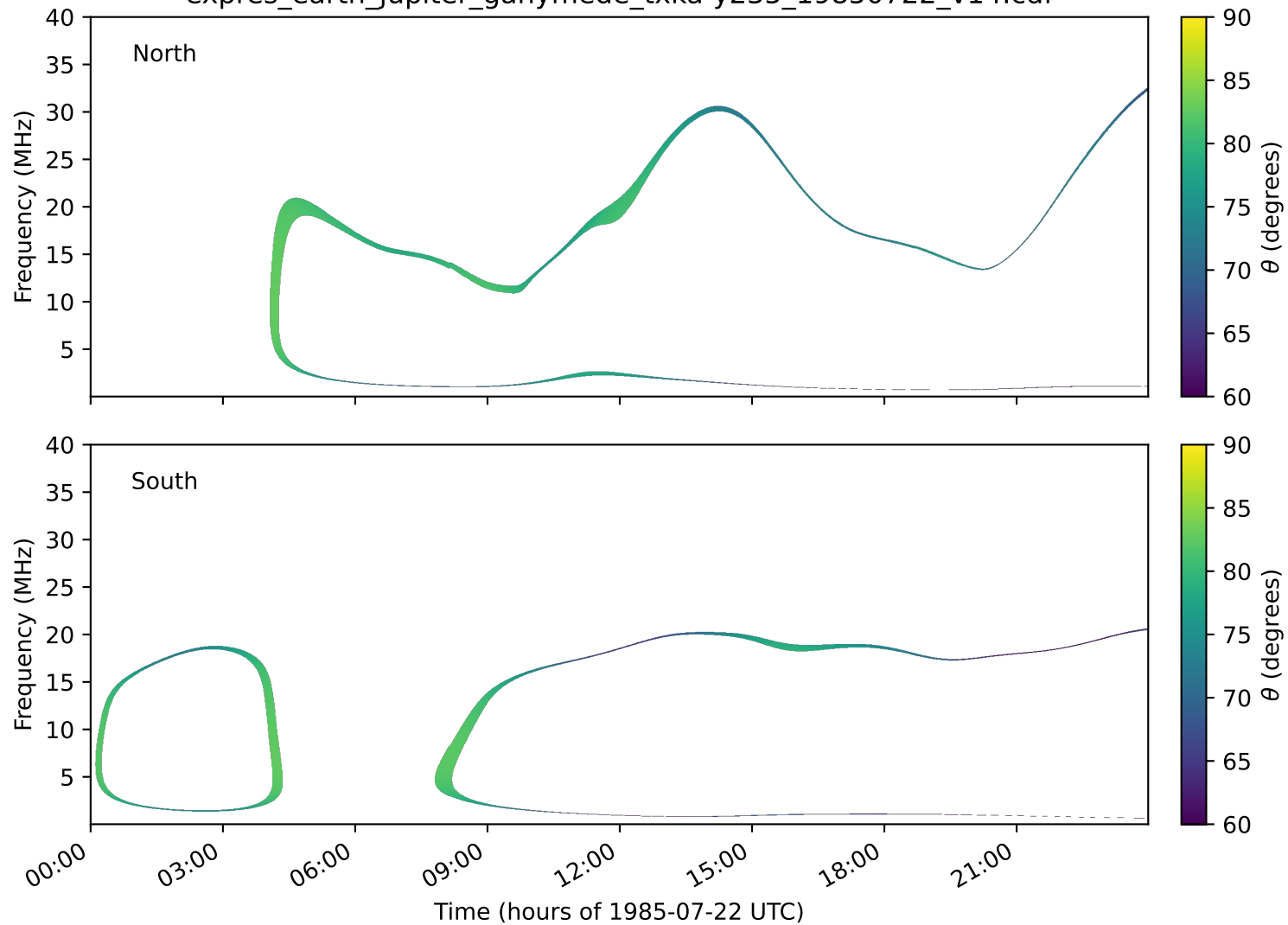
expres_earth_jupiter_ganymede_txka-y235_19850722_v14.cdf
