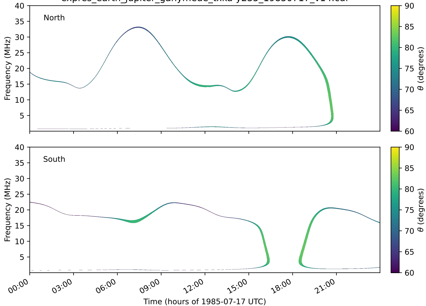
expres_earth_jupiter_ganymede_txka-y235_19850717_v14.cdf
