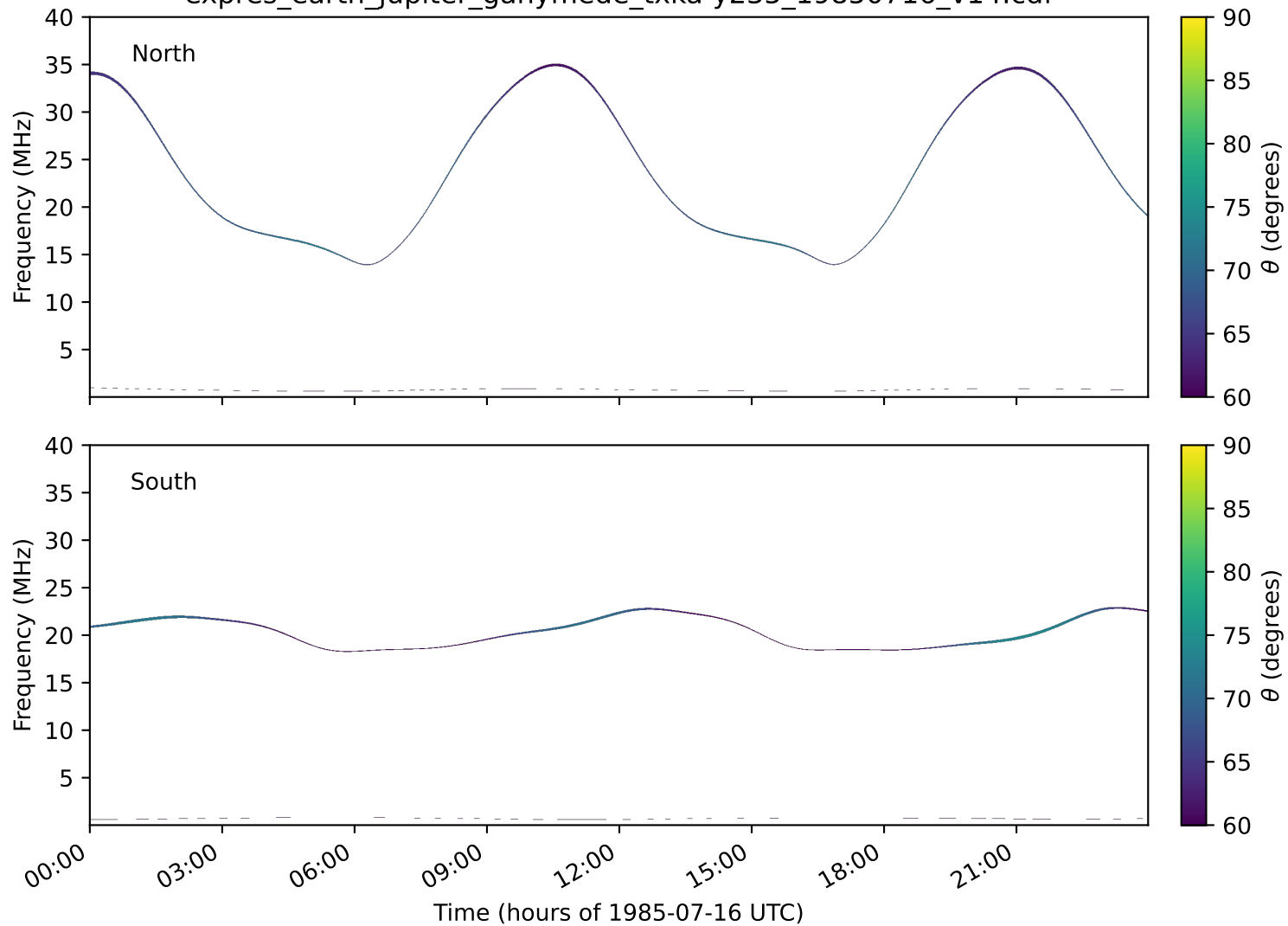
expres_earth_jupiter_ganymede_txka-y235_19850716_v14.cdf
