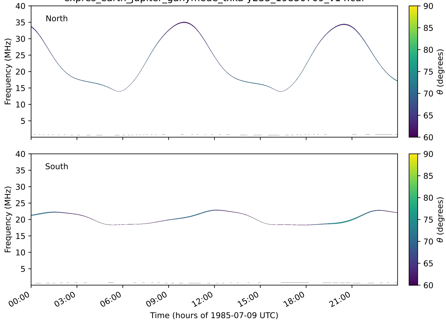
expres_earth_jupiter_ganymede_txka-y235_19850709_v14.cdf
