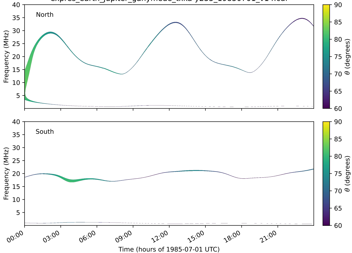
expres_earth_jupiter_ganymede_txka-y235_19850701_v14.cdf
