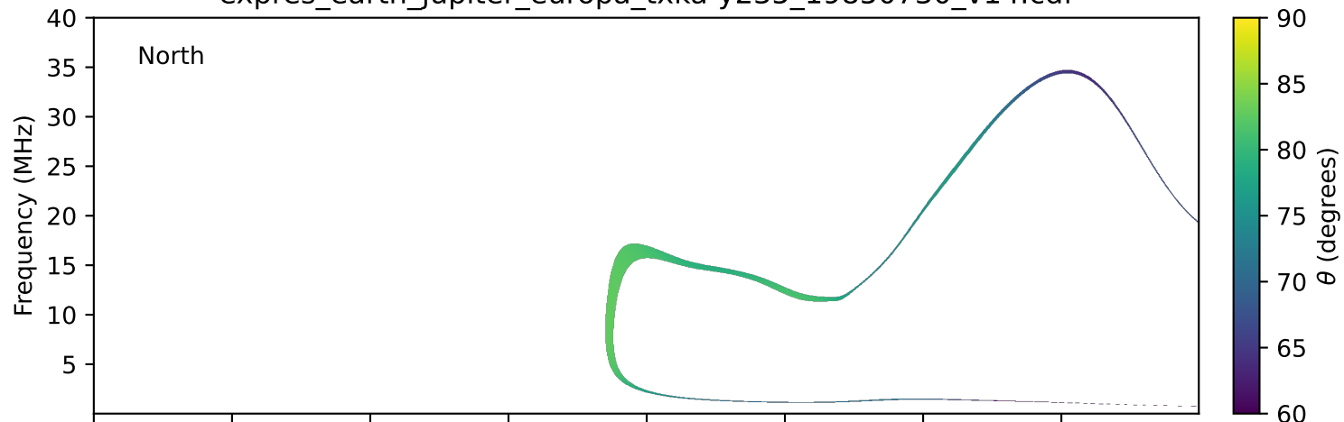
expres_earth_jupiter_europa_txka-y235_19850730_v14.cdf
