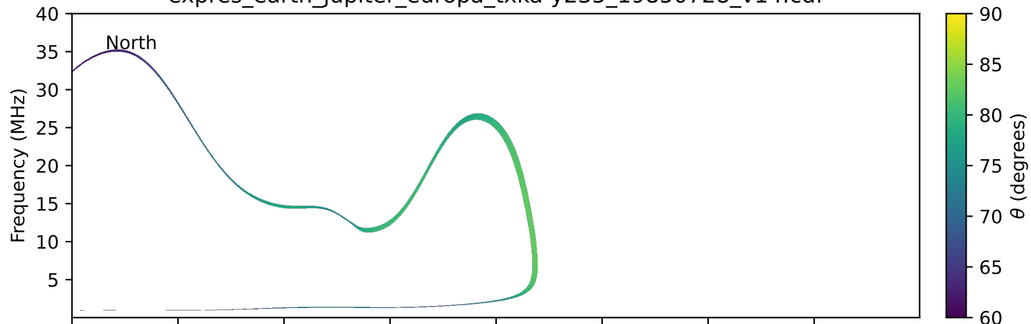
expres_earth_jupiter_europa_txka-y235_19850728_v14.cdf
