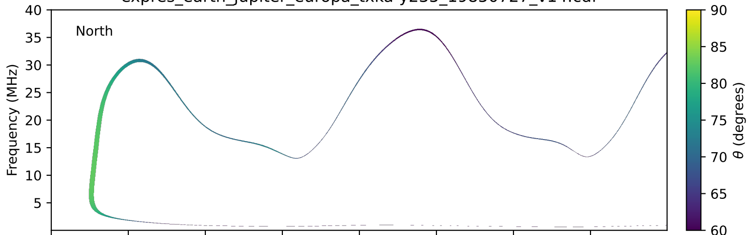
expres_earth_jupiter_europa_txka-y235_19850727_v14.cdf
