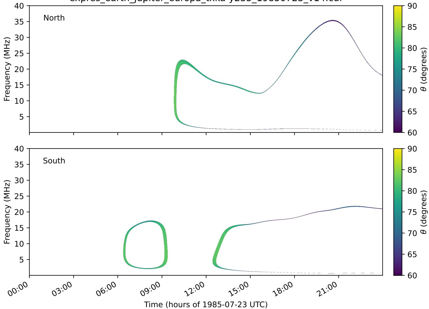
expres_earth_jupiter_europa_txka-y235_19850723_v14.cdf
