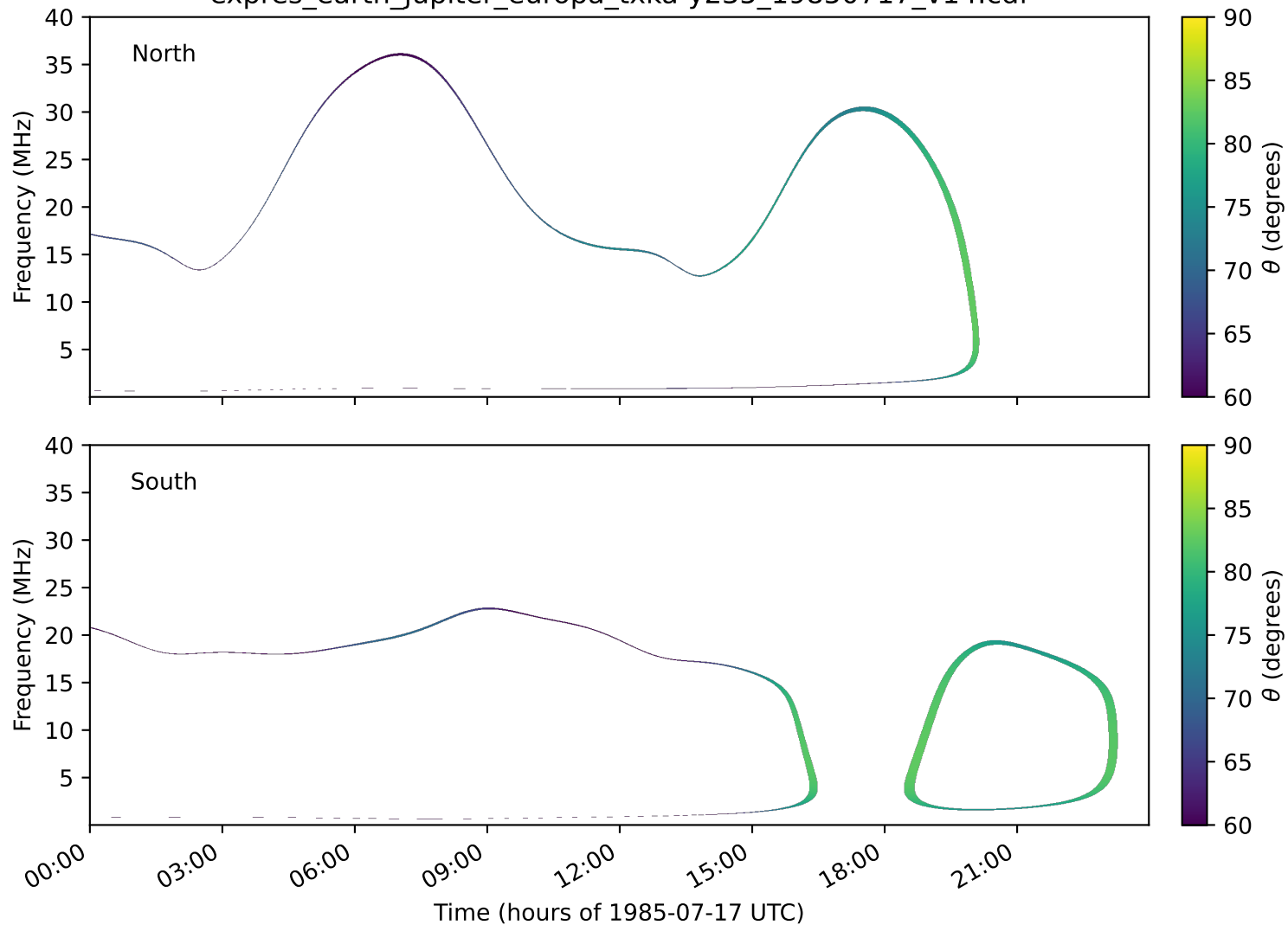
expres_earth_jupiter_europa_txka-y235_19850717_v14.cdf
