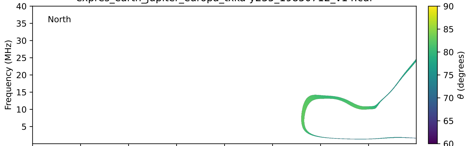
expres_earth_jupiter_europa_txka-y235_19850712_v14.cdf
