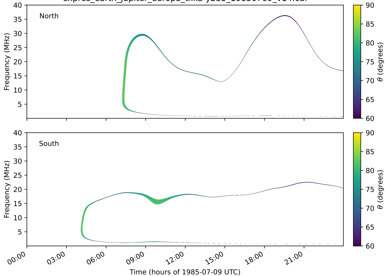
expres_earth_jupiter_europa_txka-y235_19850709_v14.cdf
