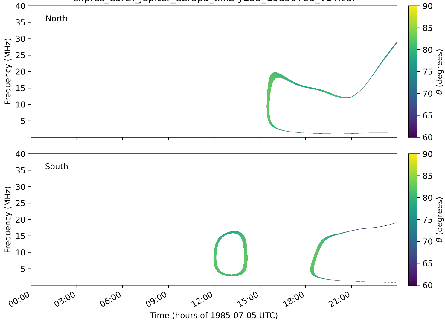
expres_earth_jupiter_europa_txka-y235_19850705_v14.cdf
