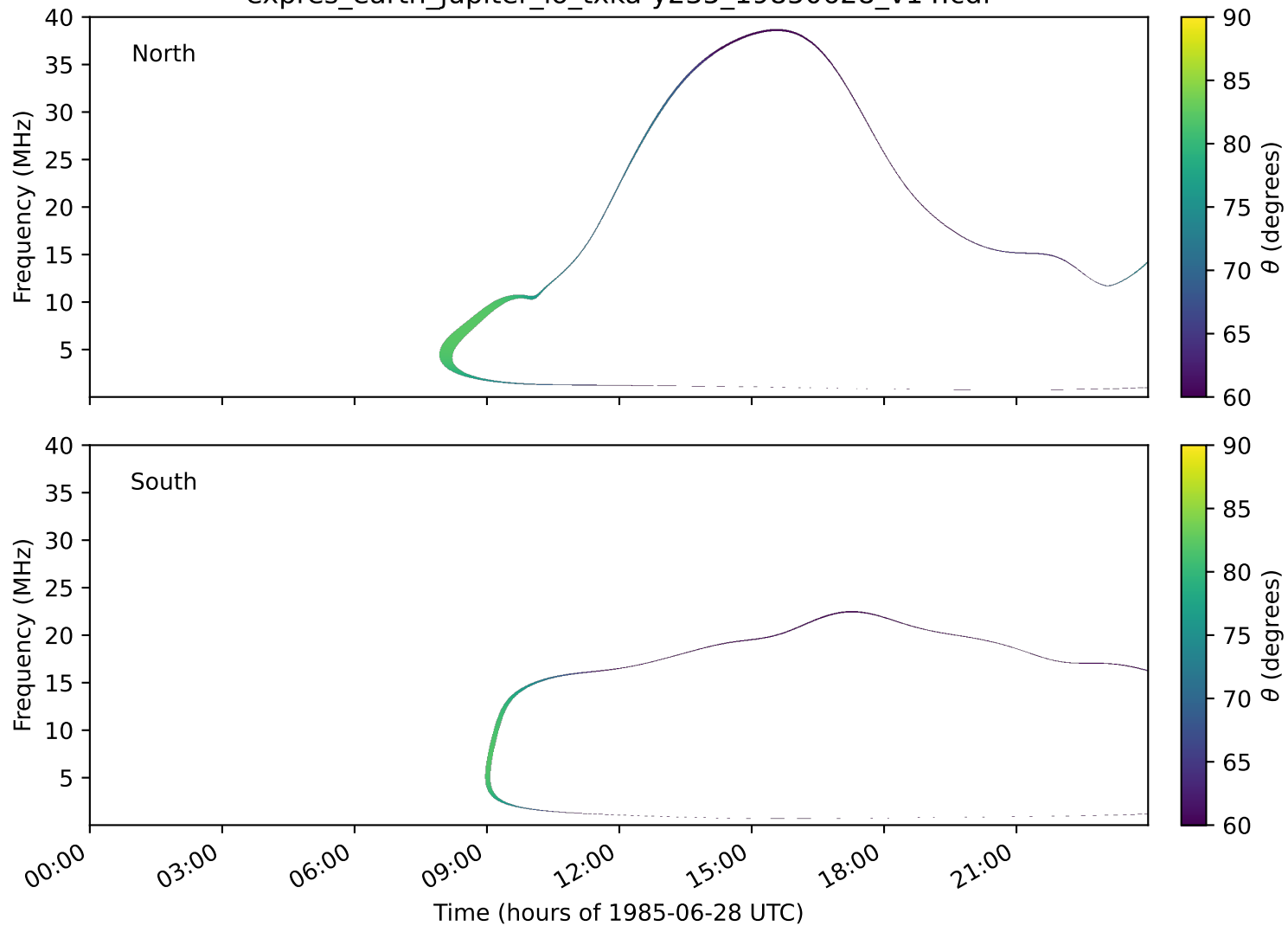
expres_earth_jupiter_io_txka-y235_19850628_v14.cdf
