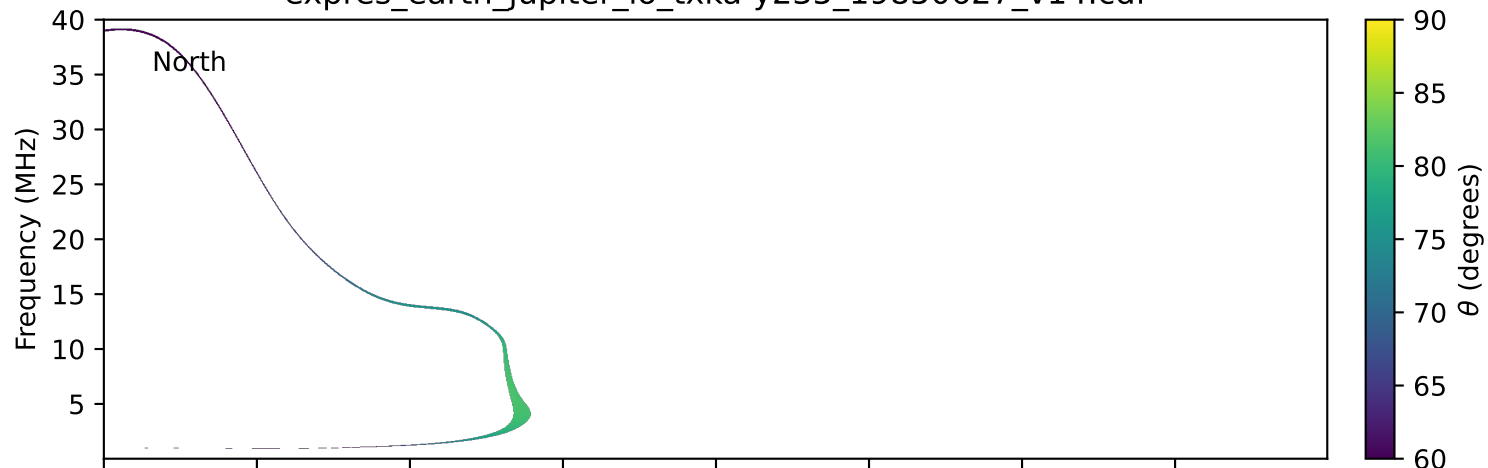
expres_earth_jupiter_io_txka-y235_19850627_v14.cdf
