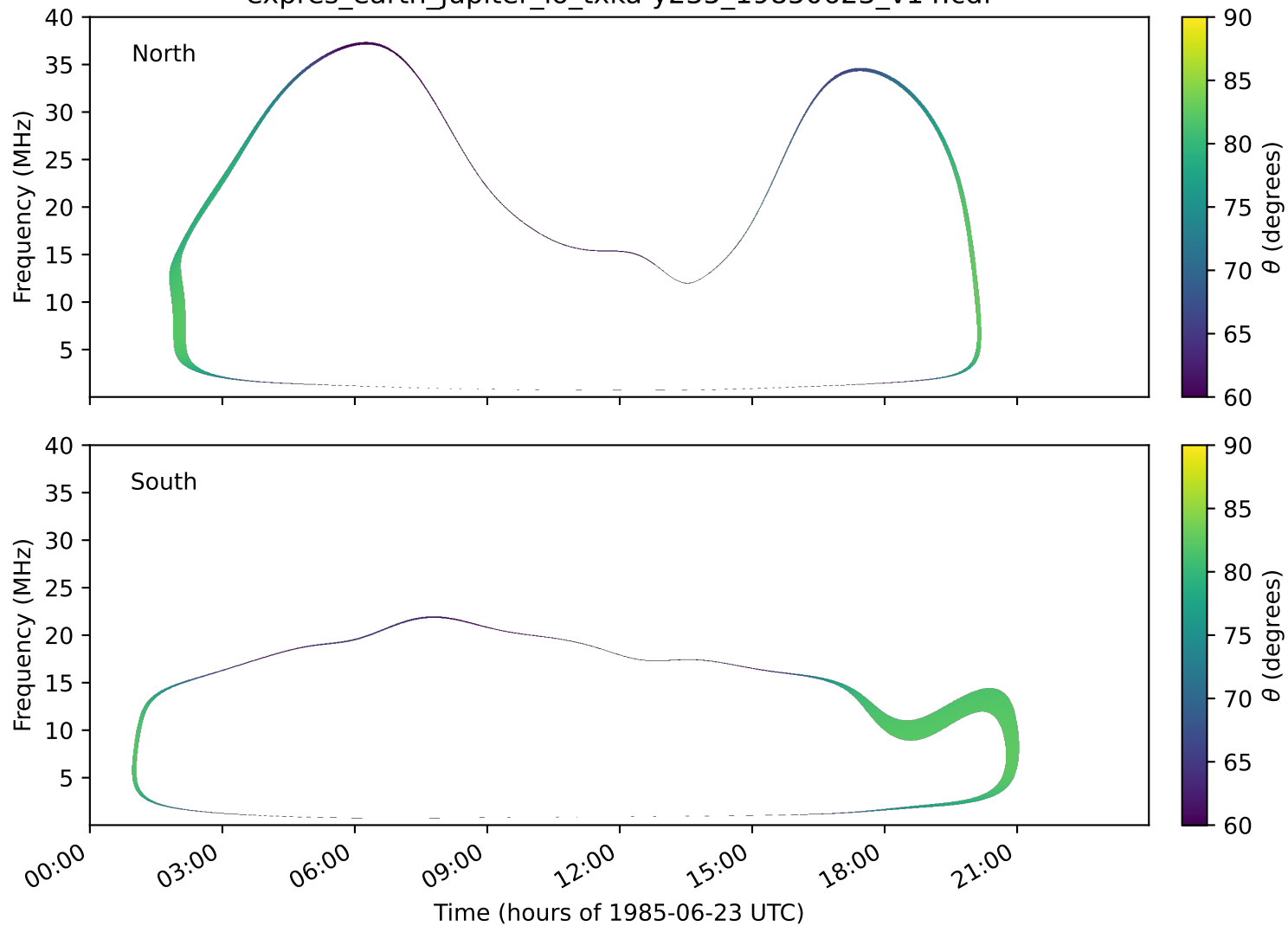
expres_earth_jupiter_io_txka-y235_19850623_v14.cdf
